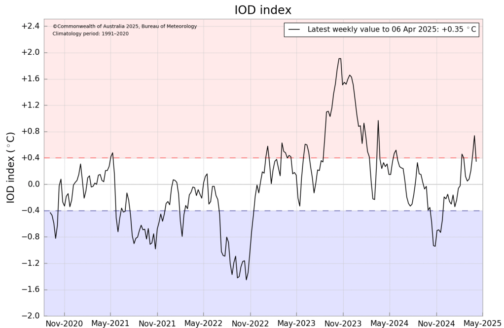
Gambar 4. Indeks DMI (Sumber: www.bom.gov.au )
