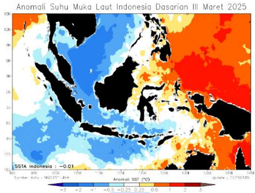
Gambar 10. Anomali SST Dasarian III Maret 2025 (sumber: www.bmkg.go.id )
